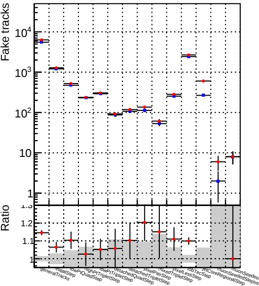
Number 1 DQM_V0001_R0000000001_Global_mkFit_jcore50maxCand-24DUPremoval-1000
