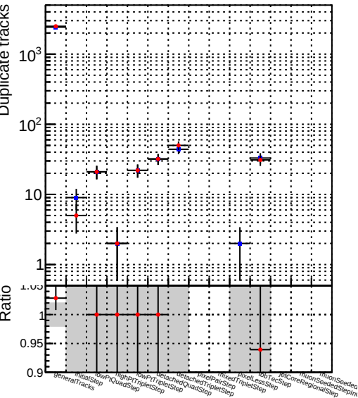
Number 1 DQM_V0001_R0000000001_Global_mkFit_jcore50maxCand-24DUPremoval-1000
