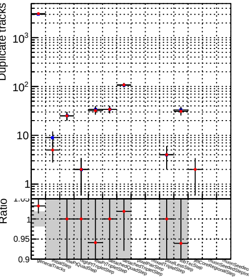
Number ● DQM_V0001_R000000001_Global_mkFit_jcore50maxCand-24DUPremoval-1000
