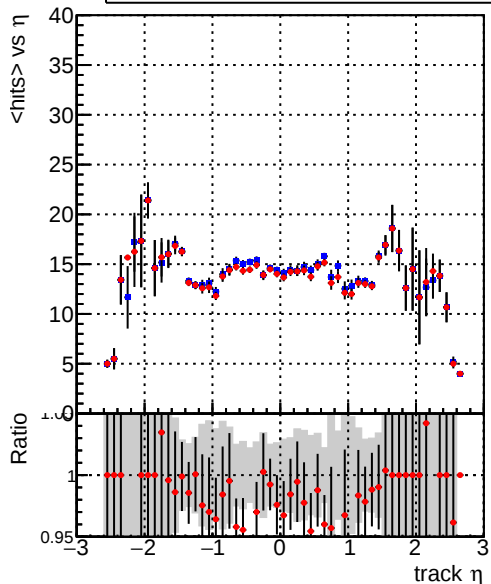
DQM_V0001_R000000001_Global_mkFit_core50maxCand-24DUPremoval-1000
