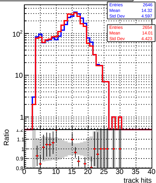
DQM_V0001_R000000001_Global_mkFit_core50maxCand-24DUPremoval-1000
