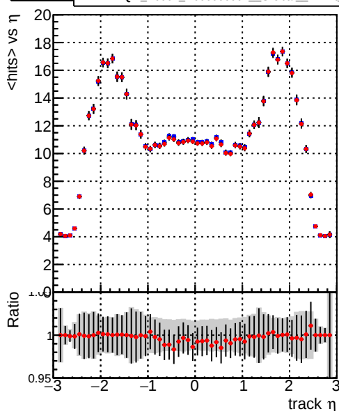
DQM_V0001_R000000001_Global_mkFit_core50maxCand-24DUPremoval-1000
