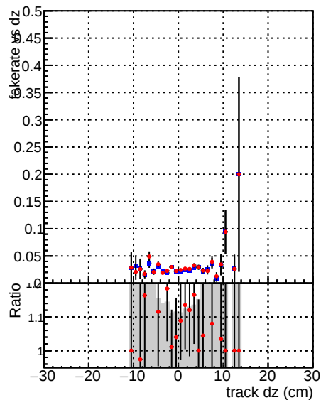
Fake rate vs dz Legend: DQM V0001_R000000001 Global mkFit baseline DQM V0001_R000000001 Global mkFit jcore50maxCand-24DUPremoval-1000
