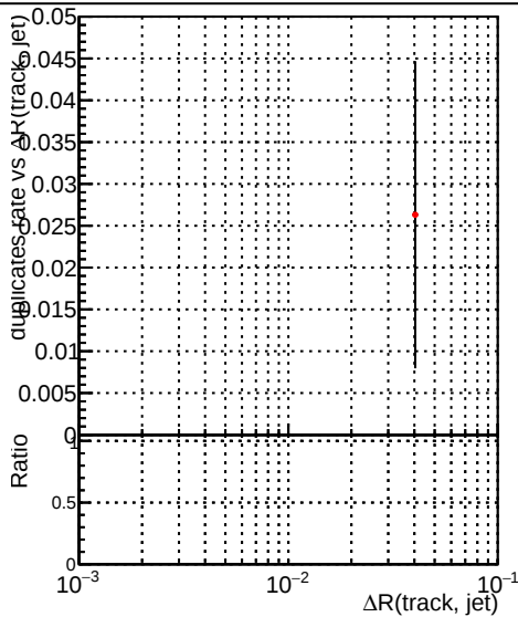
—•— DQM_V0001_R000000001_Global_mkFit_baseline —•— DQM_V0001_R000000001_Global_mkFit_jcore50maxCand-24DUPremoval-1000
