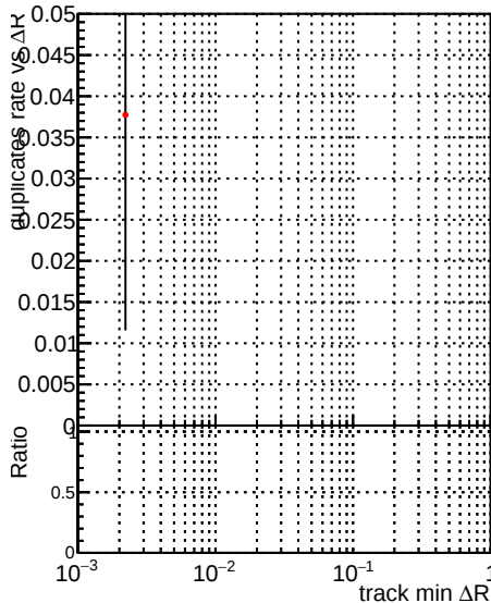
—•— DQM_V0001_R000000001_Global_mkFit_baseline —•— DQM_V0001_R000000001_Global_mkFit_jcore50maxCand-24DUPremoval-1000
