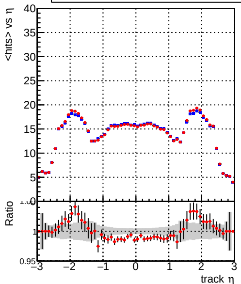
mean hits — DQM_V0001_R000000001_Global_mkFit_baseline — DQM_V0001_R000000001_Global_mkFit_core50maxCand-24DUPremoval-1000
