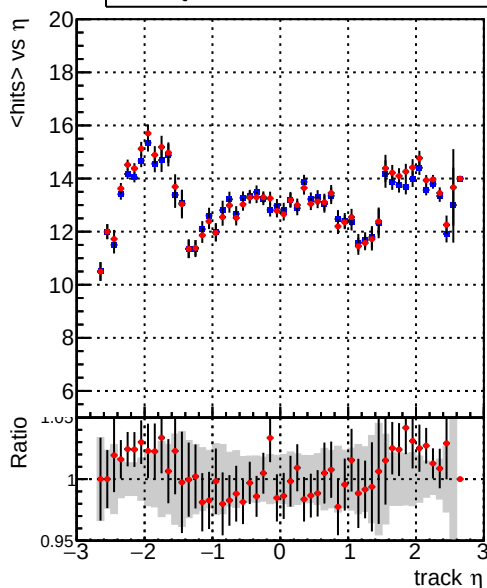
DQM_V0001_R000000001_Global_mkFit_core50maxCand-24DUPremoval-1000
