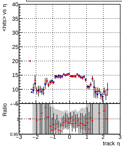
mean hits vs \eta Legend: DQM_V0001_R0000000001_Global_mkFit_baseline (blue line), DQM_V0001_R0000000001_Global_mkFit_core50maxCand-24DUPremoval-1000 (red line)
