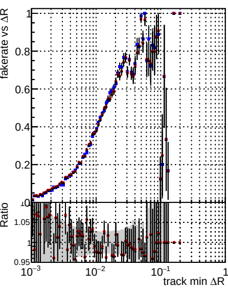
Legend: - \bullet DQM_V0001_R000000001 Global mkFit baseline - \bullet DQM_V0001_R000000001 Global mkFit_jcore50maxCand-24DUPremoval-1000 - \bullet DQM_V0001_R000000001 Global mkFit_jcore50maxCand-24DUPremoval-1000-2
