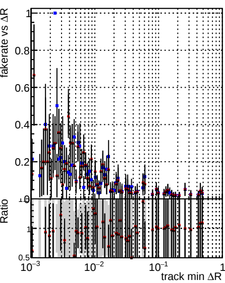
Legend: DQM_V0001_R000000001 Global mkFit_baseline, DQM_V0001_R000000001 Global mkFit_core50maxCand-24DUPremoval-1000, DQM_V0001_R000000001 Global mkFit_core50maxCand-24DUPremoval-1000-2
