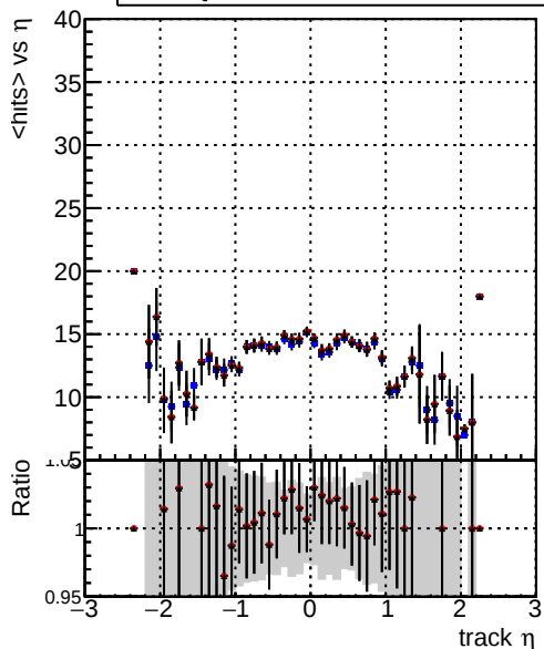
mean hits DQM_V0001_R000000001_Global_mkFit_baseline DQM_V0001_R000000001_Global_mkFit_core50maxCand-24DUPremoval-1000 DQM_V0001_R000000001_Global_mkFit_core50maxCand-24DUPremoval-1000-2
