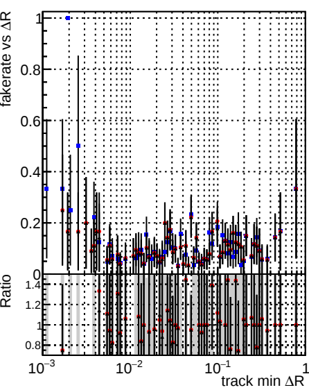
Legend: Global mkFit baseline (blue dots), Global mkFit_jcore50maxCand-24DUPremoval-1000 (red dots), Global mkFit_jcore50maxCand-24DUPremoval-1000-2 (black dots)
