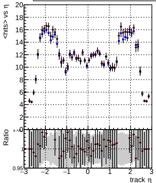
mean hits vs \eta DQM_V0001_R0000000001_Global_mkFit_baseline DQM_V0001_R0000000001_Global_mkFit_core50maxCand-24DUPremoval-1000 DQM_V0001_R0000000001_Global_mkFit_core50maxCand-24DUPremoval-1000-2
