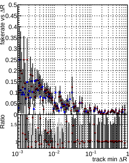
Legend: DQM_V0001_R000000001 Global mkFit baseline, DQM_V0001_R000000001 Global mkFit_jcore50maxCand-24DUPremoval-1000-2, DQM_V0001_R000000001 Global mkFit_jcore50maxCand-24DUPremoval-1000-2
