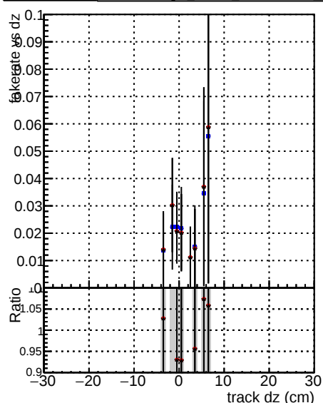
Fake rate vs dz Legend: DOM V0001 R0000000001 Global mkFit baseline DOM V0001 R0000000001 Global mkFit [core50maxCand-24DUPremoval-1000-2] DOM V0001 R0000000001 Global mkFit [core50maxCand-24DUPremoval-1000-2]
