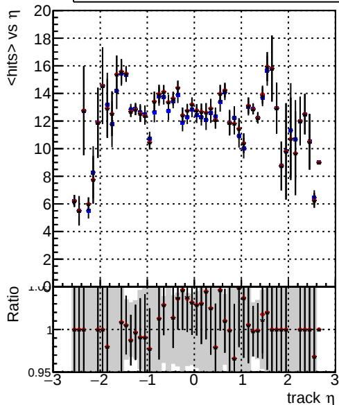
mean hits vs \eta — DQM_V0001_R0000000001_Global_mkFit_baseline — DQM_V0001_R0000000001_Global_mkFit_core50maxCand-24DUPremoval-1000 — DQM_V0001_R0000000001_Global_mkFit_core50maxCand-24DUPremoval-1000-2
