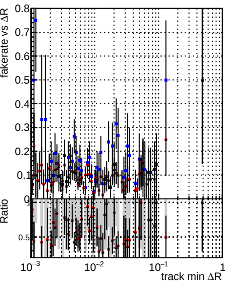
Fake rate vs \Delta R(\text{track, jet}) Legend: DQM_V0001_R000000001 Global mkFit_baseline DQM_V0001_R000000001 Global mkFit_core50maxCand-24DUPremoval-1000-2 DQM_V0001_R000000001 Global mkFit_core50maxCand-24DUPremoval-1000-2
