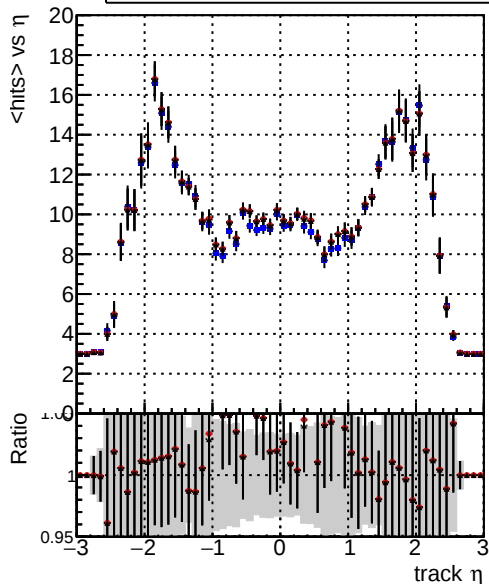
mean hit DQM_V0001_R0000000001_Global_mkFit_baseline DQM_V0001_R0000000001_Global_mkFit_core50maxCand-24DUPremoval-1000 DQM_V0001_R0000000001_Global_mkFit_core50maxCand-24DUPremoval-1000-2
