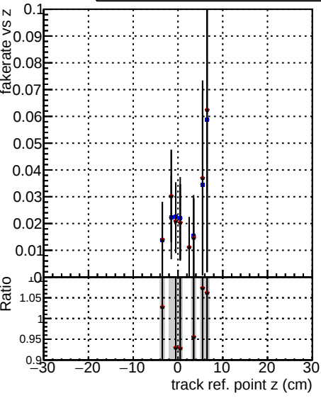
Legend: Global mkFit baseline (blue dots), Global mkFit_jcore50maxCand-24DUPremoval-1000 (red dots), Global mkFit_jcore50maxCand-24DUPremoval-1000-2 (black dots)
