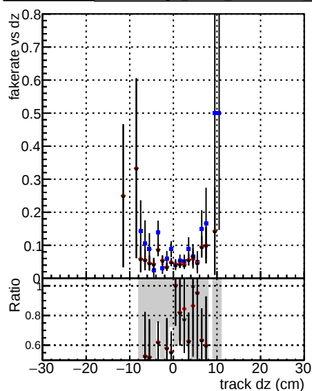
Legend for Fake rate vs dz, Duplicates Rate vs Dxy, and Pileup rate vs dxy plots: DOM V0001 R0000000001 Global mkFit baseline DOM V0001 R0000000001 Global mkFit [core50maxCand-24DUPremoval-1000-2] DOM V0001 R0000000001 Global mkFit [core50maxCand-24DUPremoval-1000-2]
