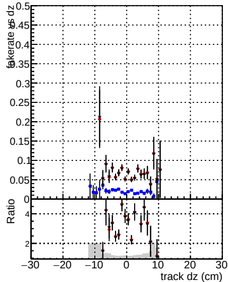
Fake rate vs dz Legend: DOM V0001 R0000000001 Global mkFit baseline DOM V0001 R0000000001 Global mkFit (core50maxCand-24DUPremoval-1000-2
