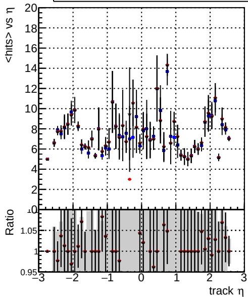
mean hit DQM_V0001_R0000000001_Global_mkFit_baseline DQM_V0001_R0000000001_Global_mkFit_jcore50maxCand-24DUPremoval-1000 DQM_V0001_R0000000001_Global_mkFit_jcore50maxCand-24DUPremoval-1000-2
