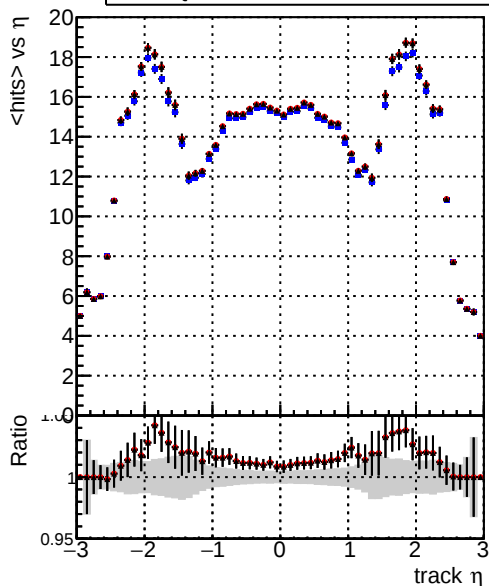
mean hits — DQM_V0001_R000000001_Global_mkFit_baseline — DQM_V0001_R000000001_Global_mkFit_core50maxCand-24DUPremoval-1000 — DQM_V0001_R000000001_Global_mkFit_core50maxCand-24DUPremoval-1000-2
