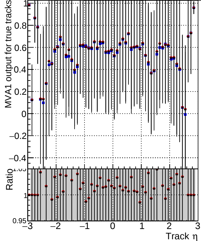
MVA1 of associated tracks (recoToSim) vs. track \eta Legend: Blue square: DQM_V0001_R0000000001_Global_mkFit_baseline Red circle: DQM_V0001_R0000000001_Global_mkFit_jcore50maxCand-24DUPremoval-1000 Black triangle: DQM_V0001_R0000000001_Global_mkFit_jcore50maxCand-24DUPremoval-1000-2
