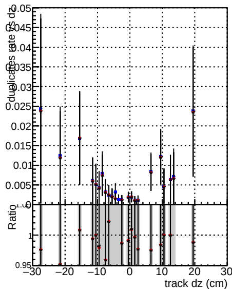
DOM V0001 R0000000001 Global mkFit baseline DOM V0001 R0000000001 Global mkFit [core50maxCand-24DUPremoval-1000-2]
