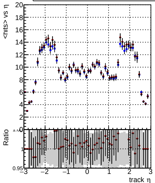
mean hits vs \eta Legend: - DQM_V0001_R000000001_Global_mkFit_baseline (blue line) - DQM_V0001_R000000001_Global_mkFit_core50maxCand-24DUPremoval-1000 (red line) - DQM_V0001_R000000001_Global_mkFit_core50maxCand-24DUPremoval-1000-2 (black line)
