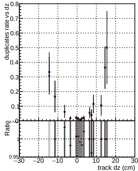
Legend for Fake rate vs d, Duplicates rate vs dz, and Pileup rate vs dz plots: DOM V0001 R0000000001 Global mkFit baseline DOM V0001 R0000000001 Global mkFit [core50maxCand-24DUPremoval-1000-2] DOM V0001 R0000000001 Global mkFit [core50maxCand-24DUPremoval-1000-2]
