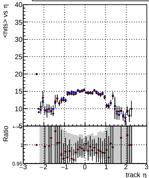
mean hits vs \eta DQM_V0001_R0000000001_Global_mkFit_baseline DQM_V0001_R0000000001_Global_mkFit_core50maxCand-24DUPremoval-1000 DQM_V0001_R0000000001_Global_mkFit_core50maxCand-24DUPremoval-1000-2
