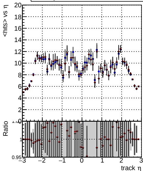
mean hits vs \eta Legend: Blue line: DQM_V0001_R000000001_Global_mkFit_baseline Red line: DQM_V0001_R000000001_Global_mkFit_core50maxCand-24DUPremoval-1000 Black line: DQM_V0001_R000000001_Global_mkFit_core50maxCand-24DUPremoval-1000-2
