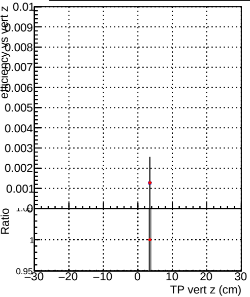
Efficiency vs vertpos Legend: DQM_V0001_R0000000001_Global_mkFit100PIXLLNO_RECO DQM_V0001_R0000000001_Global_mkFit100PIXLL_RECO
