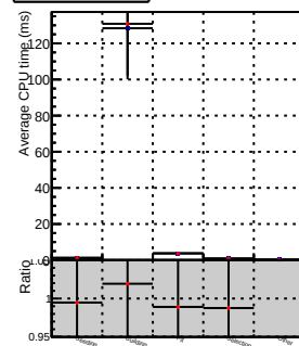
jetCoreRegionalStep
