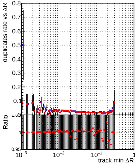
—●— DQM_V0001_R000000001_Global_mkFit100PIXLLNO_RECO —●— DQM_V0001_R000000001_Global_mkFit100PIXLL_RECO
