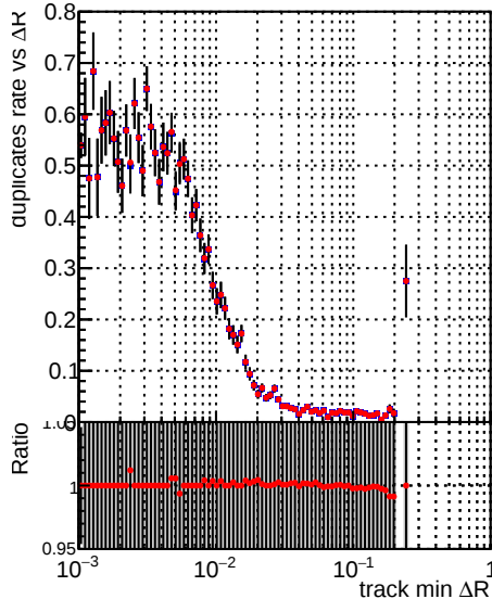
—●— DQM_V0001_R000000001_Global_mkFit100PIXLLNO_RECO —●— DQM_V0001_R000000001_Global_mkFit100PIXLL_RECO
