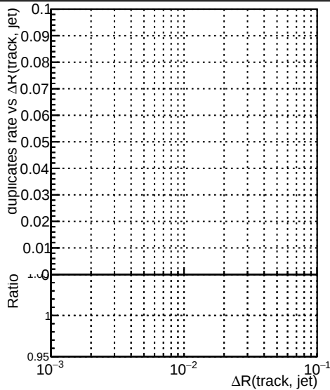
—●— DQM_V0001_R000000001_Global_mkFit100PIXLLNO_RECO —●— DQM_V0001_R000000001_Global_mkFit100PIXLL_RECO
