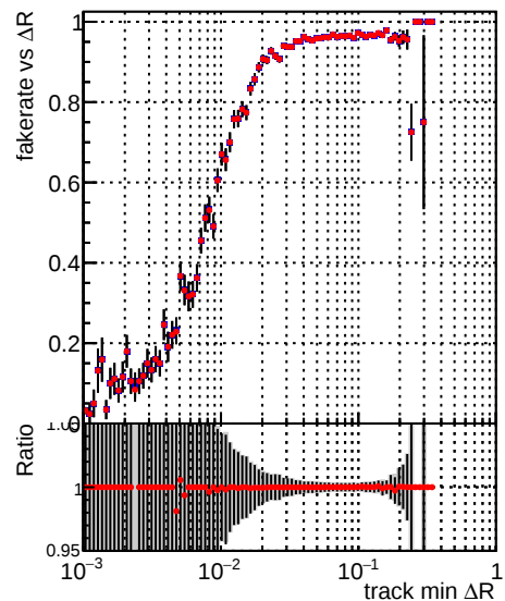
—●— DQM_V0001_R000000001_Global_mkFit100PIXLLNO_RECO —●— DQM_V0001_R000000001_Global_mkFit100PIXLL_RECO
