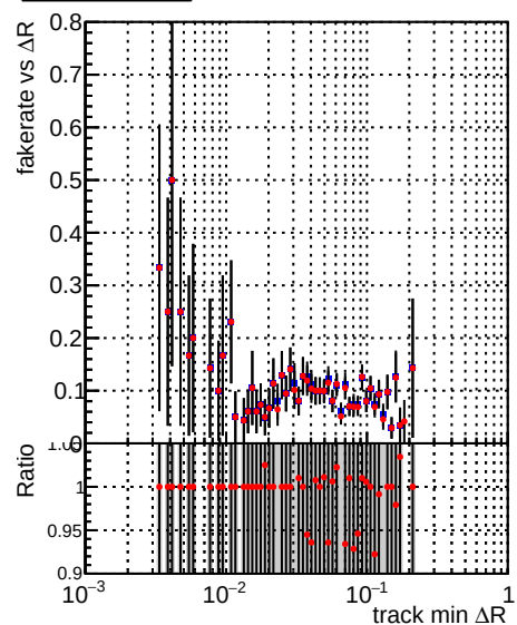
—●— DQM_V0001_R000000001_Global_mkFit100PIXLLNO_RECO —●— DQM_V0001_R000000001_Global_mkFit100PIXLL_RECO
