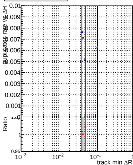
—●— DQM_V0001_R000000001_Global_mkFit100PIXLLNO_RECO —●— DQM_V0001_R000000001_Global_mkFit100PIXLL_RECO
