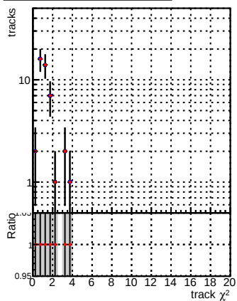
N of reco track vs. \chi^2 — Global_mkFit100PIXLLN0_RECO — Global_mkFit100PIXLL_RECO
