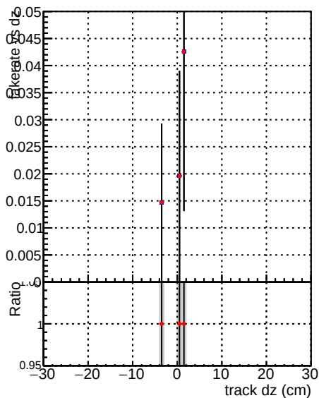
█ █ DQM_V0001_R0000000001_Global mkFit100PIXLLNO_RECO █ █ DQM_V0001_R0000000001_Global mkFit100PIXLL_RECO
