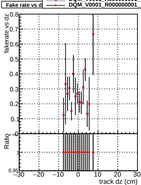
—•— DQM_V0001_R0000000001_Global_mkFit100PIXLLNO_RECO —•— DQM_V0001_R0000000001_Global_mkFit100PIXLL_RECO
