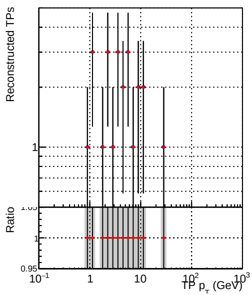
Legend: DQM_V0001_R000000001_Global_mkFit100PIXLLNO_RECO (blue line), DQM_V0001_R000000001_Global_mkFit100PIXLL_RECO (red line)
