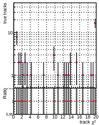
N of reco track vs. \chi^2 for DQM_V0001_R0000000001_Global_mkFit100PIXLLNO_RECO (black) and DQM_V0001_R0000000001_Global_mkFit100PIXLL_RECO (red)
