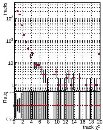
N of reco track vs. \chi^2 —●— DQM_V0001_R0000000001_Global_mkFit100PIXLLNO_RECO —●— DQM_V0001_R0000000001_Global_mkFit100PIXLL_RECO
