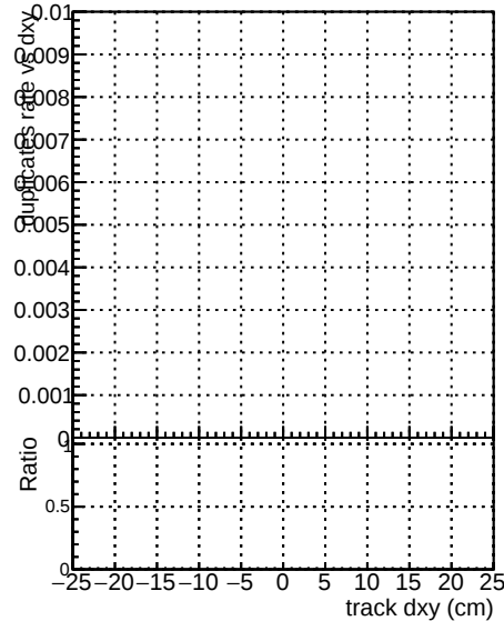
DQM_V0001_R0000000001 Global mkFit100PIXLLNO RECO Fake rate vs d Blue dot Blue line Blue line Blue line Duplicates Rate vs Dxy Red dot Red line Red line Red line
