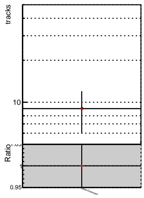
Global_mkFit100PIXLLNO_RECO Global_mkFit100PIXLL_RECO
