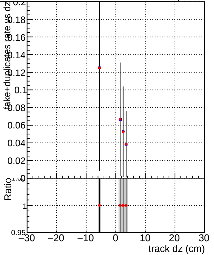
DQM_V0001_R000000001_Global_mkFit100PIXLLNO_RECO DQM_V0001_R000000001_Global_mkFit100PIXLL_RECO
