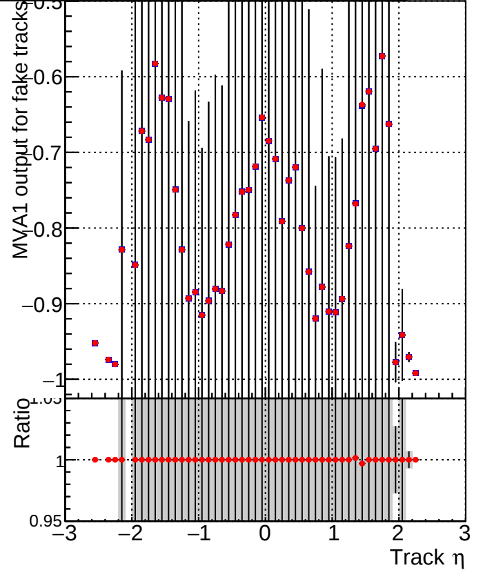
MVA1 of associated tracks (recoToSim) vs. track \eta Legend: ■ DQM_V0001_R000000001_Global_mkFit100PIXLLNO_RECO ● DQM_V0001_R000000001_Global_mkFit100PIXLL_RECO
