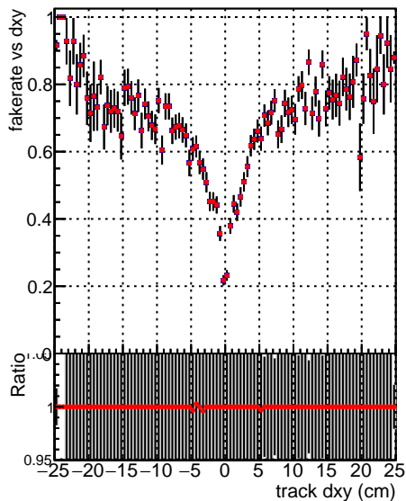
—●— DQM_V0001_R000000001_Global_mkFit100PIXLLNO_RECO —●— DQM_V0001_R000000001_Global_mkFit100PIXLL_RECO
