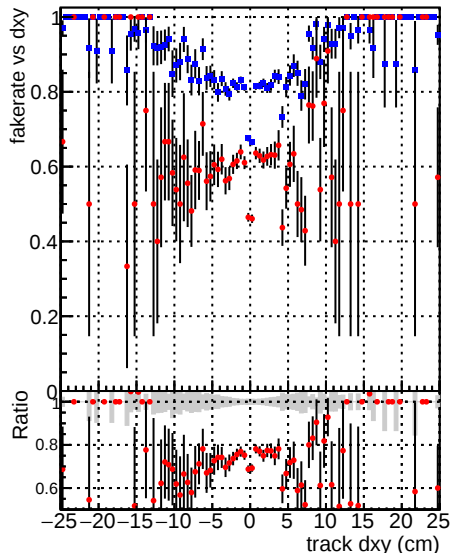
—●— DQM V0001_R000000001 Global mkFit100PIXLLNO_RECO —●— DQM V0001_R000000001 Global mkFit100PIXLLNO_RECO
