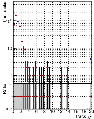
N of reco track vs. \chi^2 DQM V0001_R000000001 Global_mkFit100PIXLLN0_RECO DQM V0001_R000000001 Global_mkFit100PIXLL_RECO
