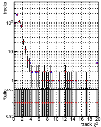
N of reco track vs. \chi^2 DQM V0001_R000000001 Global_mkFit100PIXLLN0_RECO DQM V0001_R000000001 Global_mkFit100PIXLL_RECO
