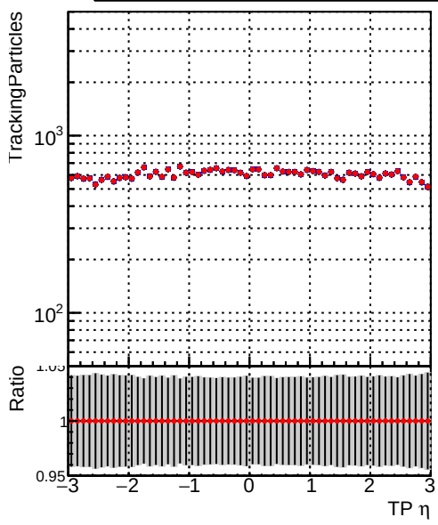
Legend: DQM_V0001_R000000001_Global_mkFit100PIXLLNO_RECO (blue line), DQM_V0001_R000000001_Global_mkFit100PIXLL_RECO (red line)
