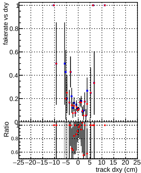
—●— DQM V0001_R000000001 Global mkFit100PIXLLNO RECO —●— DQM V0001_R000000001 Global mkFit100PIXLL RECO
